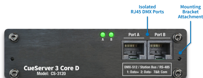
Front Panel
